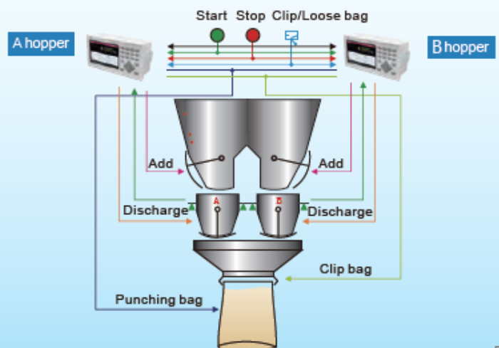
Dual channel packaging controller with hopper
